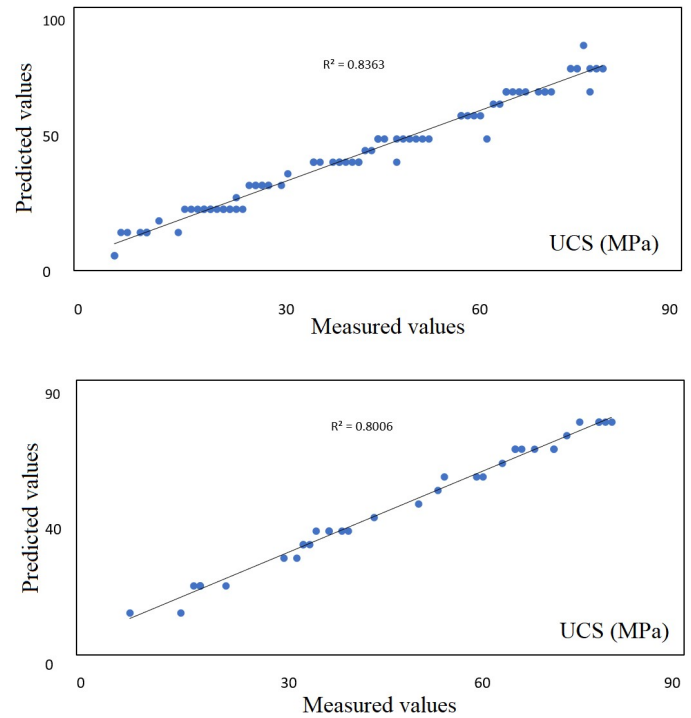
Fig. 5 Correlation between measured and predicted values for UCS with SVM
